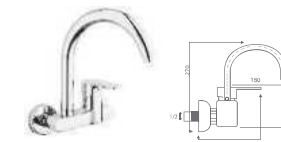
CODE: 103 21 14 32 Brass Pipe CODE: 103 20 14 33 Stainless Pipe Mix Üstten Aplike Eyye Bataryası Ø28 Borulu Sink Mixer, Applique Type Ø28 Pipe 12 PCS.
