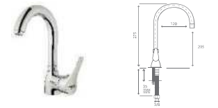
CODE: 105 08 07 34 Brass Pipe CODE: 105 09 07 35 Stainless Pipe Mix Kuğu Lavabo Bataryası Washbasin Mixer, Swan Type 12 PCS.
