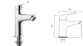
CODE: 210 18 00 00 Minox Tekli Lavabo Bataryası Minox Basin Mixer 🔧 40 PCS.
