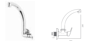
CODE: 210 11 00 42 Brass Pipe CODE: 210 12 00 43 Stainless Pipe Duvardan Tekli Mix Eyje Bataryası (Ø28) Single Washbasin Mixer, Wall Type (Ø28) 🔧 40 PCS.
