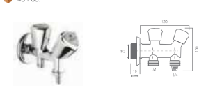
CODE: 301 21 02 00 Çift Musluk 1/2-3/4 Rekorlu Double Tap 🔧 40 PCS.
