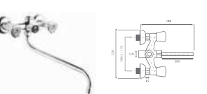
CODE: 301 12 02 18 Stainless Pipe Rus Banyo Bataryası Russian Bath Mixer 🔧 10 PCS.
